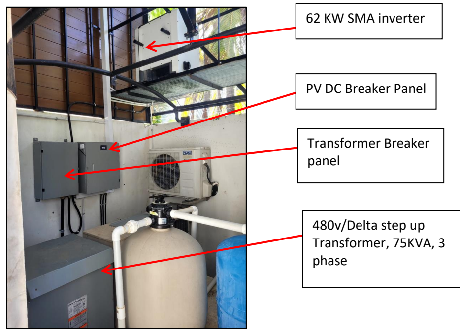
Photo #4: Overview of solar components
