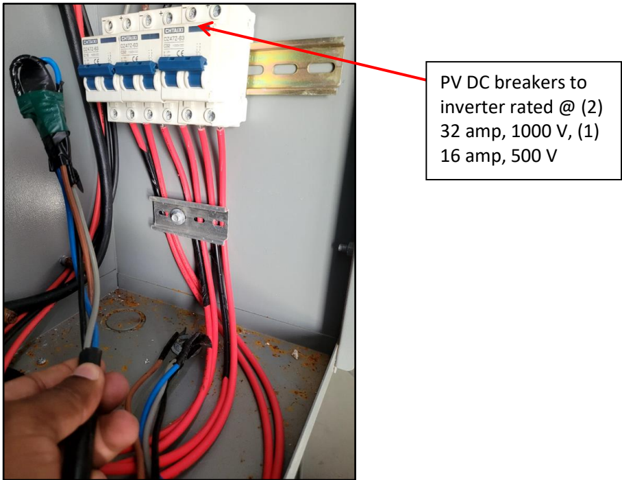
Photo #5: Overview of PV DC breakers
