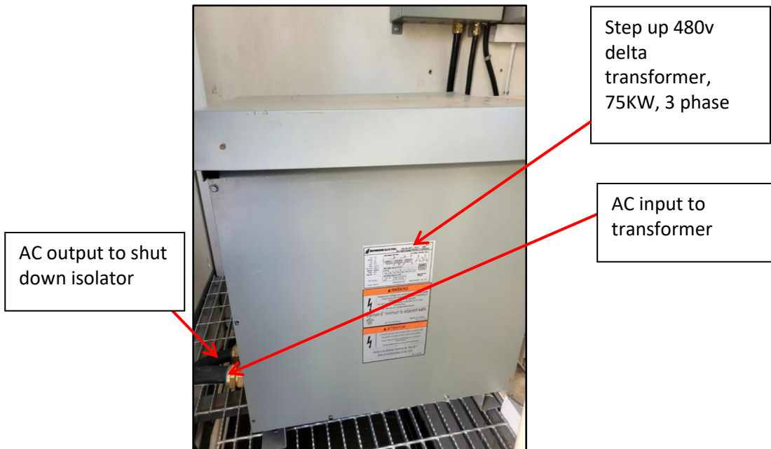
Photo #10: Overview of Step-up Transformer
